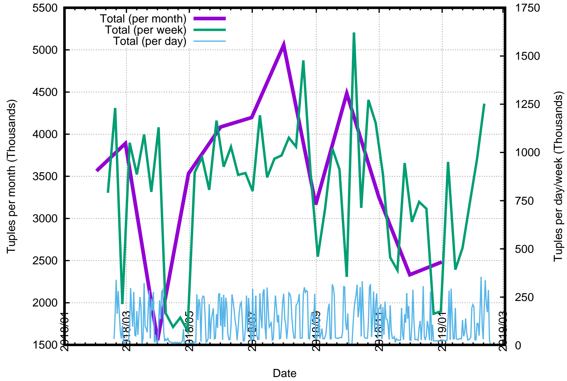
Submissions per day/week/month (1 Year Window)
